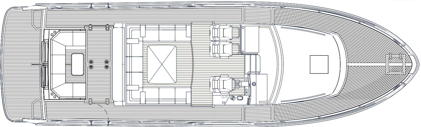
Main Deck
