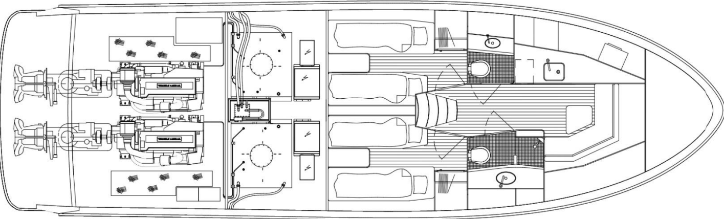
Cabin Deck
